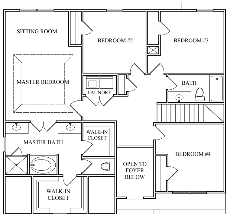
SECOND FLOOR
